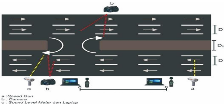
Fig. 2. Measurement metode
